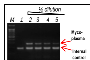
Fig. 4. Mycoplasma detection was performed for genomic DNA Lane M, 100bp DNA Marker; lane 1, Internal control; lane 2, 25pg; lane 3, 12.5pg; lane 4, 6.3pg; lane 5, 3.25pg
