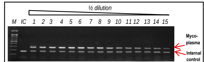
Fig.1. Mycoplasma detection was performed for genomic DNA
