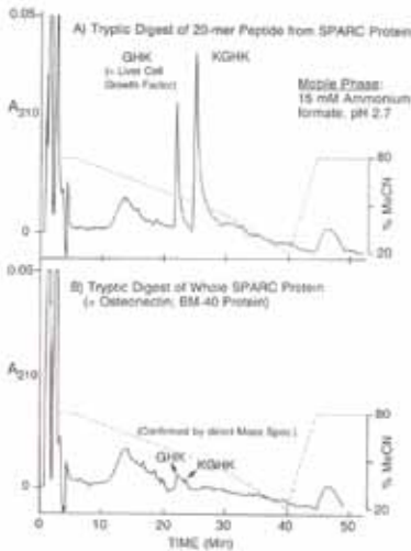
PolyHYDROXYETHYL Aspartamide™
