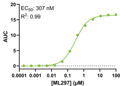
Figure 5. \text{EC}_{50} Calculation. Plot the V_{\text{max}} or the AUC against the compound concentrations and run the non-linear regression "agonist vs response" in GraphPad® Prism to calculate an \text{EC}_{50} . Alternatively, run the non-linear regression "inhibitor vs response" to calculate an \text{IC}_{50} .
