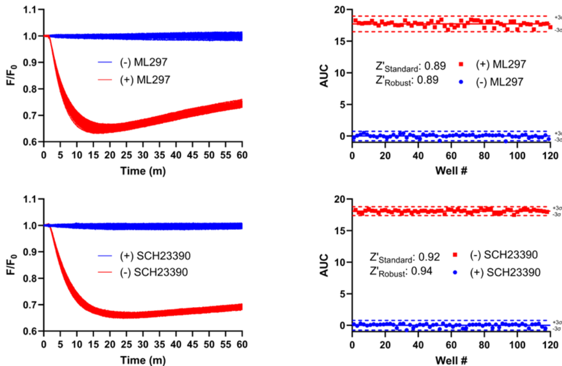
Figure 8. Z' Determination in K ir 3.1/3.2-Expressing HEK293 Cells. Baseline-normalized kinetic fluorescence data collected using Wavefront Panoptic (Excitation: 518 nm, Emission: 562(40) nm). ±SCH23390, a selective GIRK Channel inhibitor, was pre-incubated for 15 minutes at a concentration of 100 μM before the start of the assay. ±ML297, a potent activator of GIRK Channels, was added at 60 seconds at a concentration of 10 μM. The AUC was calculated between the curve and y=1. The Z' factor plots show a Z' above 0.8 for both ML297 activation and SCH23390 inhibition of K ir 3.1/3.2 (n = 60).
