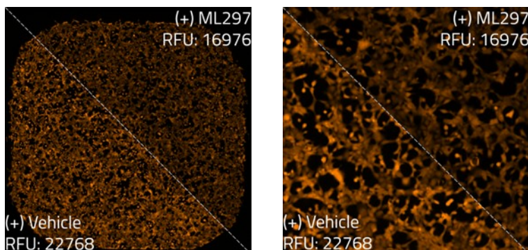
Figure 9. ML297 Activation of GIRK Channels in HEK293 Cells Expressing Kir3.1/3.2. HEK293 cells stably expressing Kir3.1/3.2 were plated in a 384-well format, incubated with Dye Loading Solution, and treated with Stimulus Solution containing ML297 or vehicle for 1 hour, resulting in a final well concentration of 10 \mu M ML297. Whole-well images were acquired using a Cytation 5 imager with a 4X objective, RFP filter (Ex: 531/40 nm, Em: 593/40 nm).
