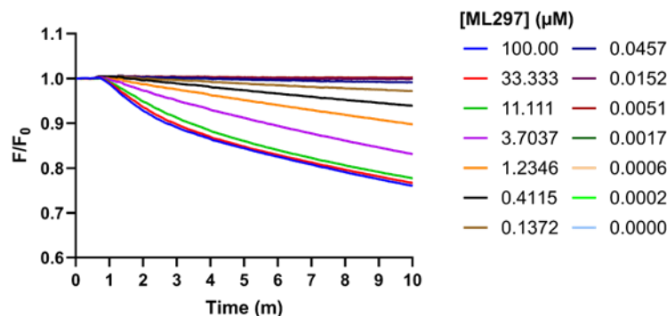
Figure 3. Baseline-Normalized Fluorescence Kinetic Data. Based on the Raw Kinetic Fluorescence Data from figure 2, average the Relative fluorescence Units (F) of the initial 60 seconds before stimulus addition as the baseline ( F_0 ). Calculate the ratio of Relative fluorescence Units (F) over F_0 at each time point as F/F_0 . Plot F/F_0 over time as the Baseline-Normalized Fluorescence Kinetic Data.
