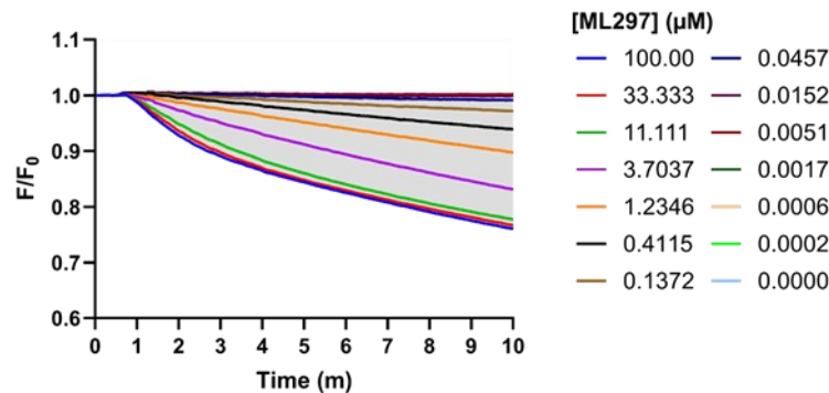
Figure 4. Area Under Curve (AUC) Calculation. Based on the Baseline-Normalized Fluorescence Kinetic Data from Figure 3, calculate the area between the curve and y=1 and define it as the AUC.
