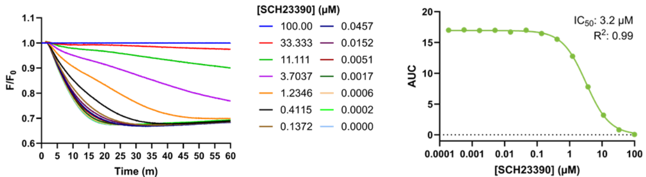
Figure 7. SCH23390 Inhibition of GIRK Channels in K ir 3.1/3.2-Expressing HEK293 Cells. Baseline-normalized kinetic fluorescence data collected using Wavefront Panoptic (Excitation: 518 nm, Emission: 562(40) nm). SCH23390, a selective GIRK channel inhibitor, was added 15 minutes before the start of the assay. ML297, a potent activator of GIRK Channels, was added at 60 seconds at a concentration of 10 μM. The AUC was calculated between the curve and y=1. Error bars indicate the SEM (n = 3). The IC 50 for SCH23390 inhibition of K ir 3.1/3.2 is about 3.2 μM.
