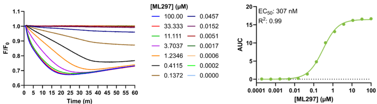
Figure 6. ML297 Activation of GIRK Channels in \text{K}_{\text{ir}}3.1/3.2 -Expressing HEK293 Cells. Baseline-normalized kinetic fluorescence data collected using Wavefront Panoptics (Excitation: 518 nm, Emission: 562(40) nm). ML297, a potent activator of GIRK Channels, was added at 60 seconds. The AUC was calculated between the curve and y=1 . Error bars indicate the SEM ( n = 3 ). The \text{EC}_{50} for ML297 activation of \text{K}_{\text{ir}}3.1/3.2 is about 307 nM.
